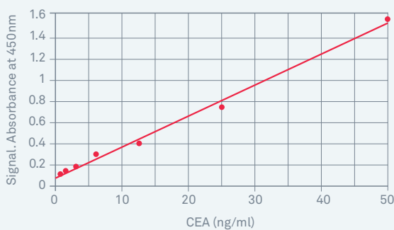
Sandwich ELISA using BM220-E1E3 as the capture antibody and BM220-D7C6 as the detection antibody. CEA antigen P824-3 was used as the standard.
