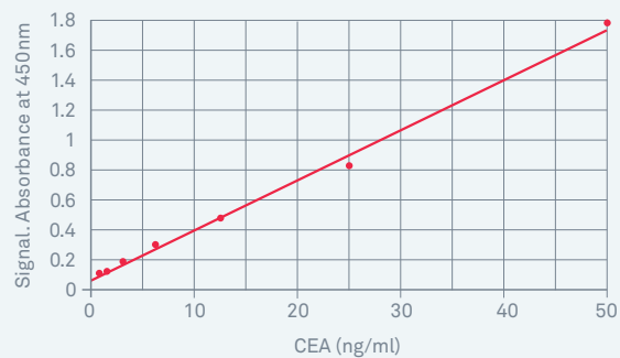
Sandwich ELISA using BM220-E1E3 as the capture antibody and BM220-E7E2 as the detection antibody. CEA antigen P824-3 was used as the standard.
